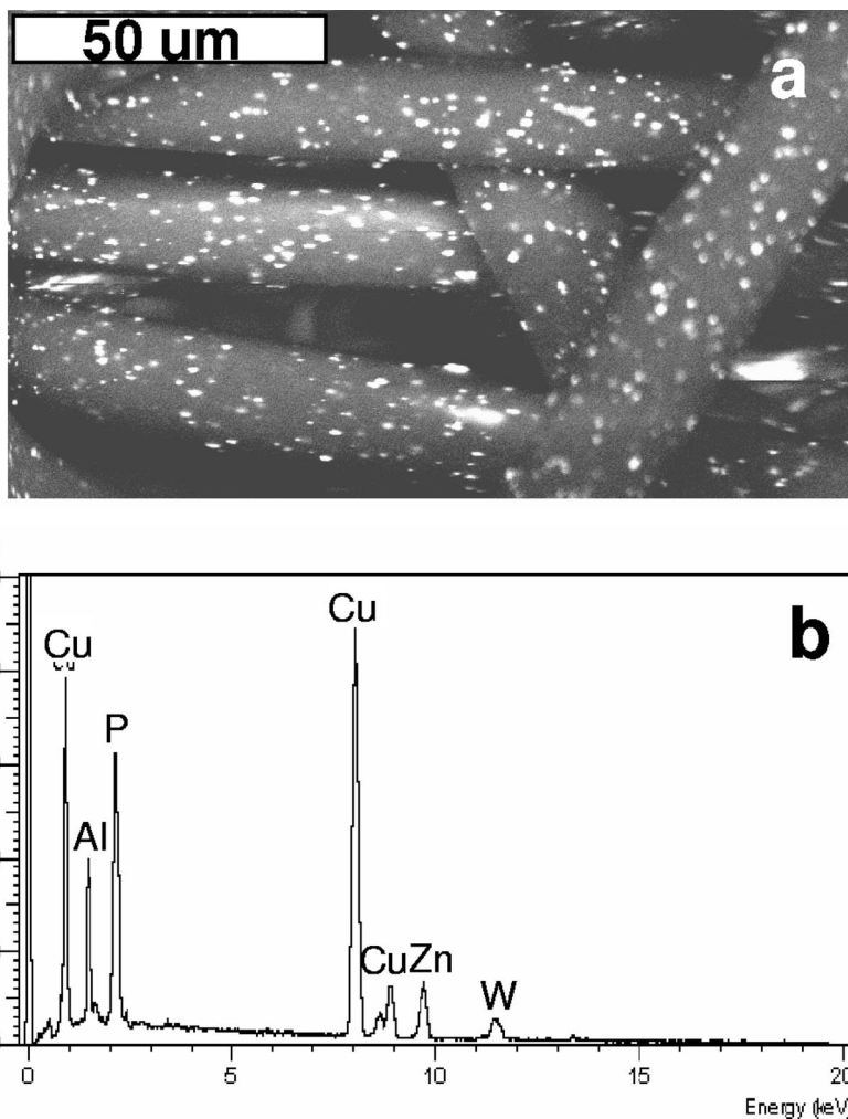
FIG. 4. Copper oxide-impregnated polypropylene fibers. (a) Scanning electron microscopy (JEOL JMS 5410 LV scanning electron microscope, Japan) of a copper oxide-impregnated polypropylene fibers. Bar, 50 \mu m. (b) X-ray photoelectron spectrum analysis (Link IV, ISIS, Oxford Instruments, England) of the surfaces of the copper-impregnated fibers used to fill filters for deactivation of HIV-1.
